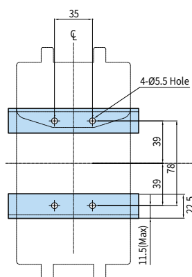
Mounting Drawing
