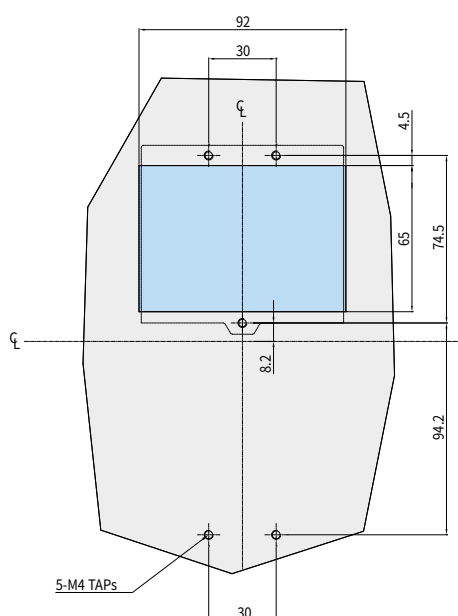
Mounting Drawing
