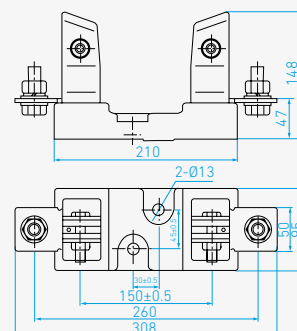
Fuse Base
