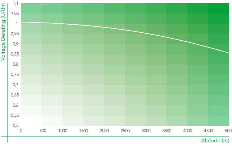
Voltage Derating vs Altitude
